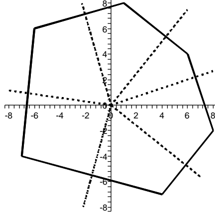
FIGURE 3. The complex conjugate convex hull for exponential sum (1.6), and the corresponding rays \mathcal{S}_{j,j+1} , j = 1, \dots, 6 .
