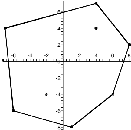
FIGURE 2. The convex hull for exponential sum (1.6), with \lambda_1 = 8 + 2i , \lambda_2 = 4 + 7i , \lambda_3 = -7 + 4i , \lambda_4 = -6 - 6i , \lambda_5 = 1 - 8i , \lambda_6 = 6 - 4i , \lambda_7 = 4 + 4i , \lambda_8 = -2 - 4i .
