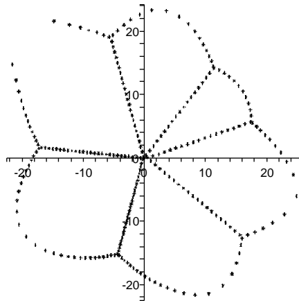
FIGURE 1. The zeros of the n = 250 section of exponential sum (1.6).
