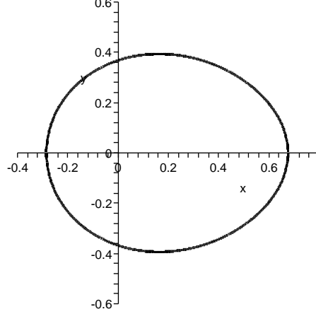
FIGURE 4. The generalized Szegő curve for c = 0.9 .
